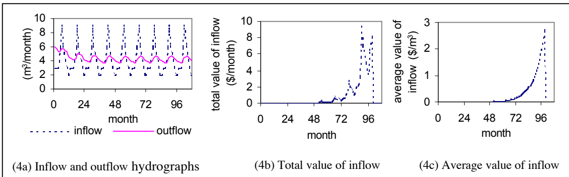
Figure 4. Transfer of water values in upstream direction in a water system with a large reservoir
