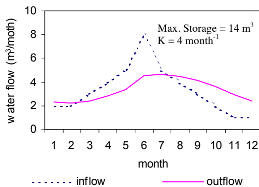
Figure 5. Inflow and outflow hydrographs before any upstream abstraction
