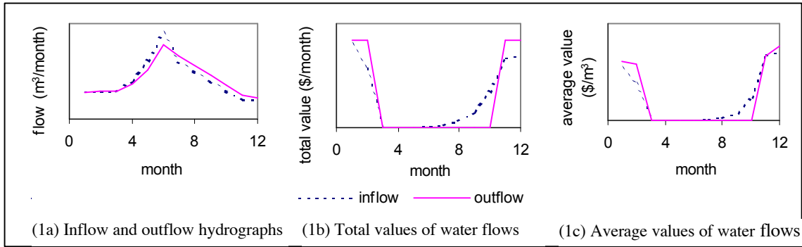
Figure 1. The translation of an inflow hydrograph into an outflow hydrograph and the translation of an outflow-value curve into an inflow-value curve in the case of a small reservoir.
