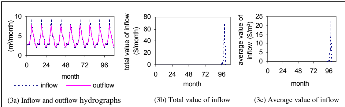
Figure 3. Transfer of water values in upstream direction in a water system with a small reservoir
