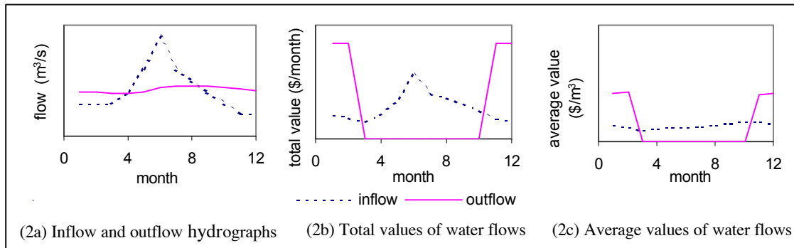
Figure 2. The translation of an inflow hydrograph into an outflow hydrograph and the translation of an outflow-value curve into an inflow-value curve in the case of a large reservoir.
