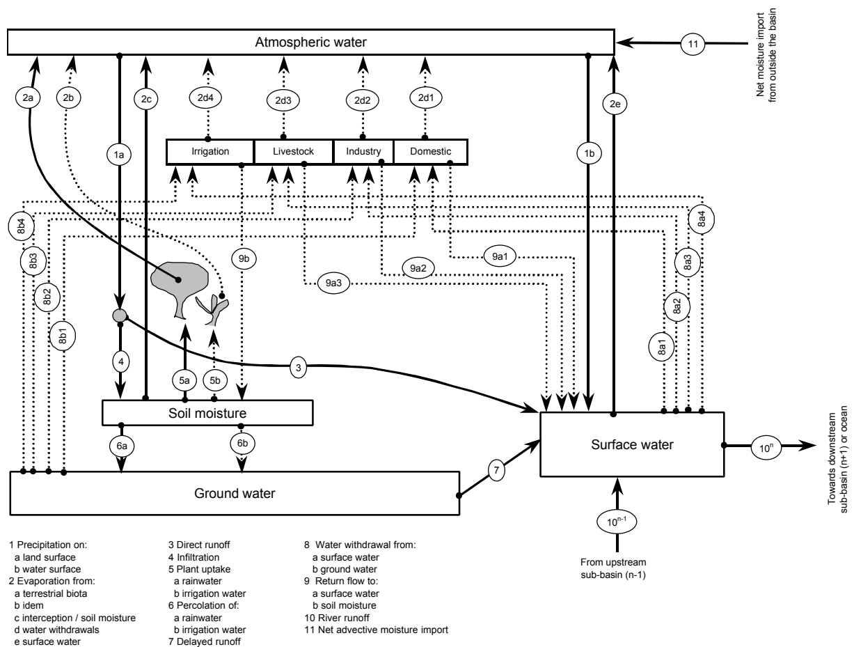
Fig. 4. Water flow schematisation within a sub-basin.
